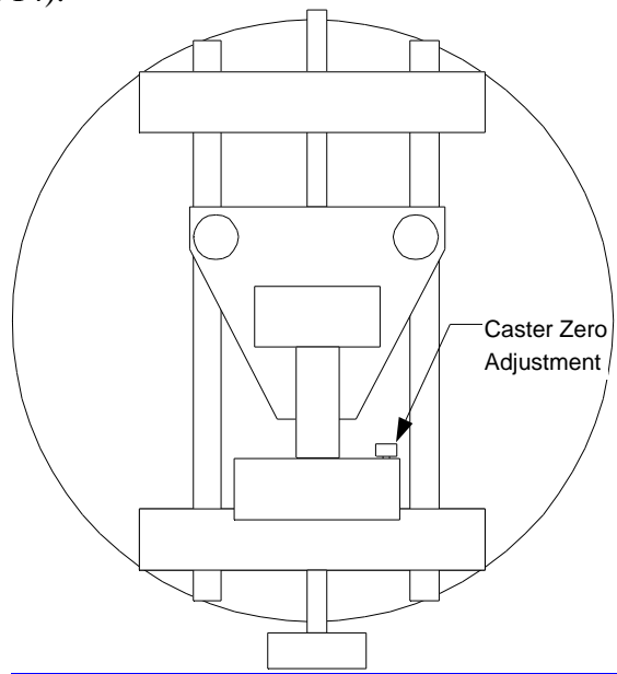
FIGURE 14 Caster Zero Adjustment= Ajuste de Caster a Cero
